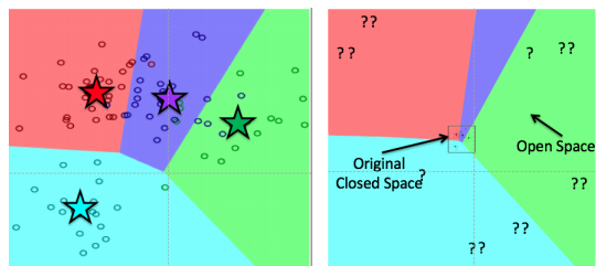
(a) Example four-class model (b) Zooming out to show from closed set point of view. some open space.
