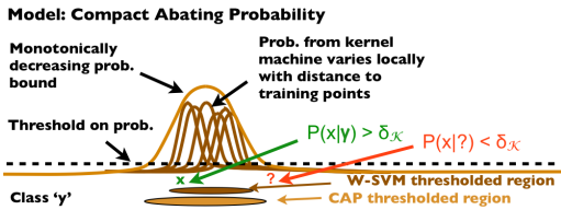
Figure 2: Compact Abating Probability (CAP) model which, when thresholded, can bound open space risk. CAP models are often used in novelty, anomaly, or outlier detectors.
